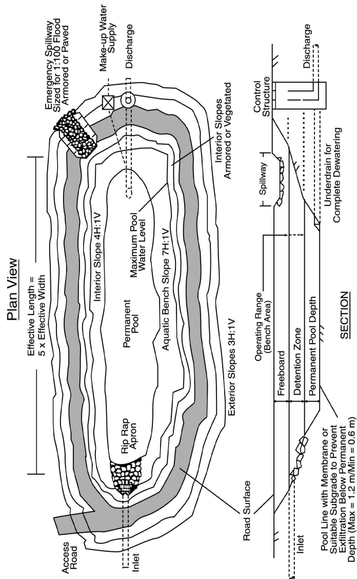
Figure 6.10 Wet Detention Pond Plan and Sections
